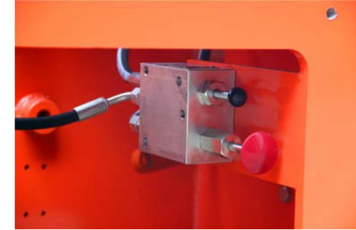
Brake release valve from White
